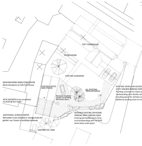
BLOCK PLAN 1:200 AT A1
