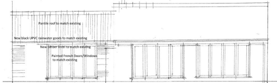
EAST ELEVATION, PROPOSED 1:50 AT A1
