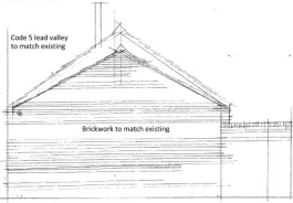
SOUTH ELEVATION, PROPOSED 1:50 AT A1
